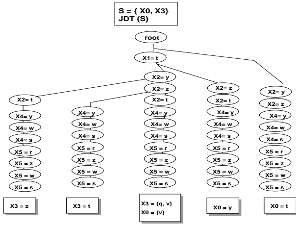
Figure 2: Joint Discrimination Tree (JDT) for set S = \{x_0, x_3\} .
